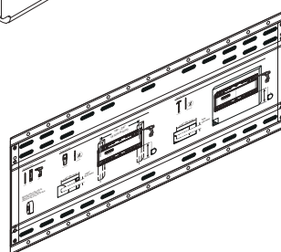
Wall Plate Template - 1pcs
