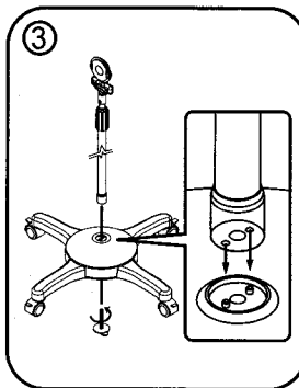
Stand assembly
